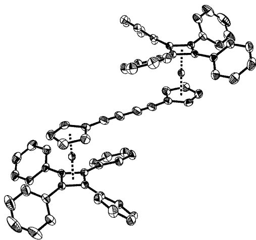
Figure 2. ORTEP plot (50% probability) of the molecular structure of 15
