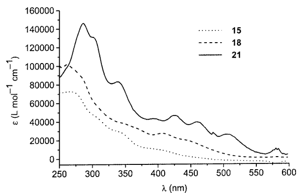
Figure 4. UV/Vis spectra of 15 , 18 , and 21
