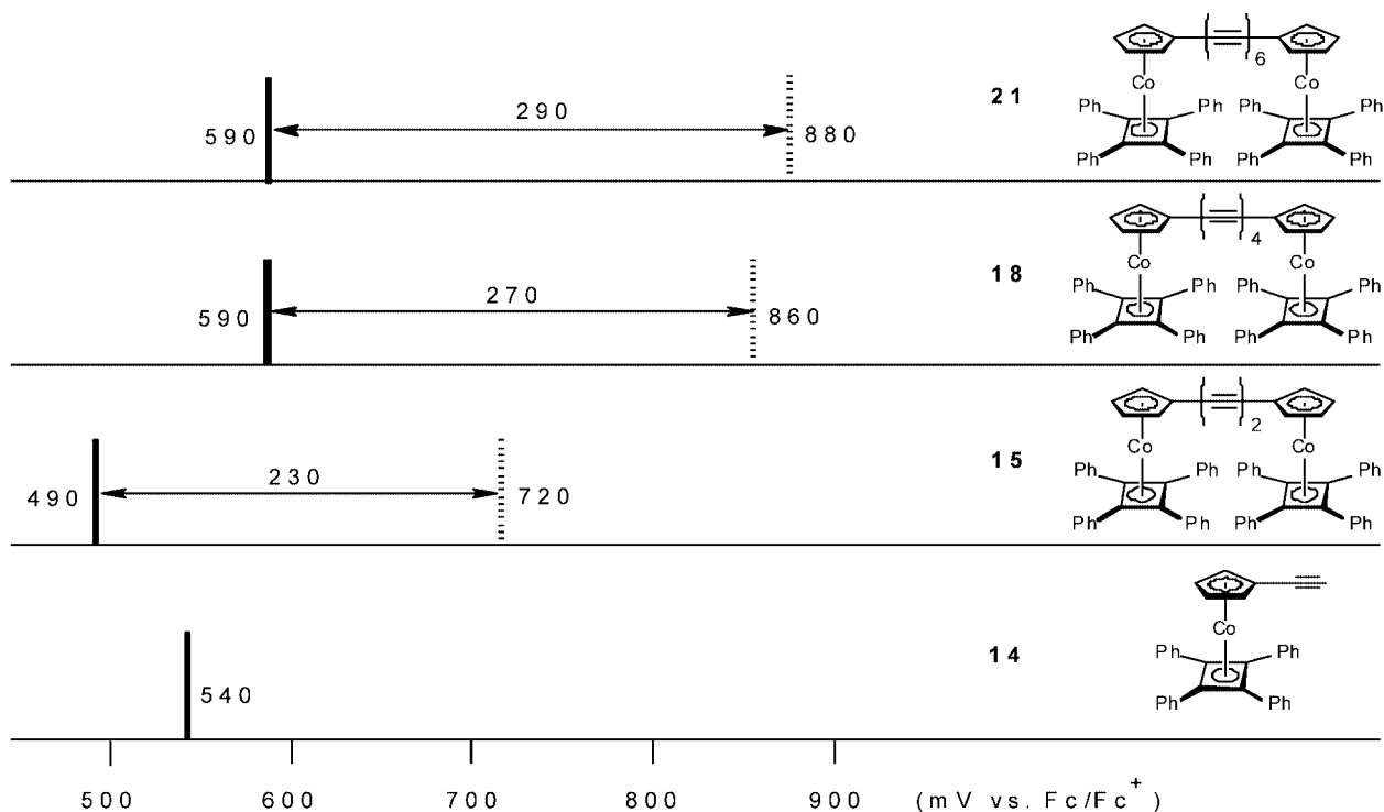
Figure 5. Comparison of the CV data of 14 , 15 , 18 , and 21
