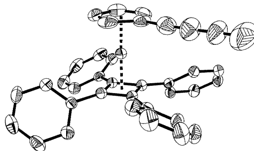
Figure 1. ORTEP plot (50% probability) of the molecular structure of 17
